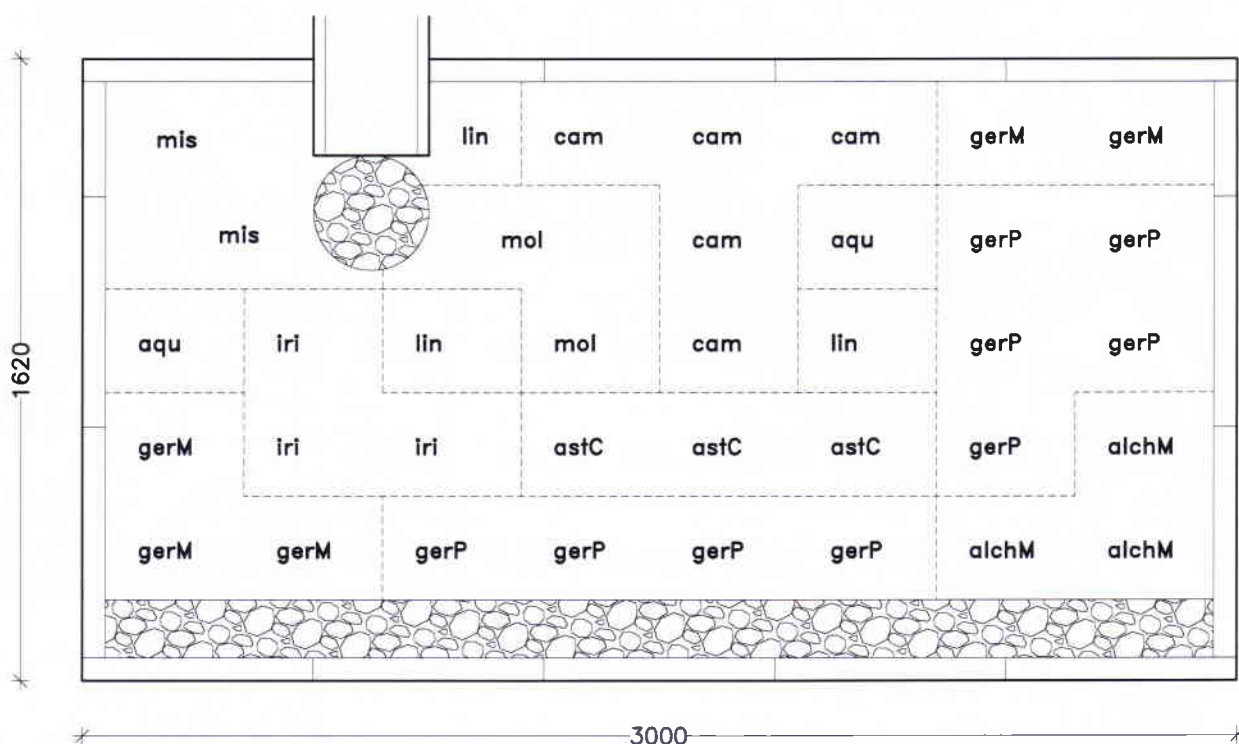
REGNBED C, STOR PRINCIP FOR REGNBED 1:20
